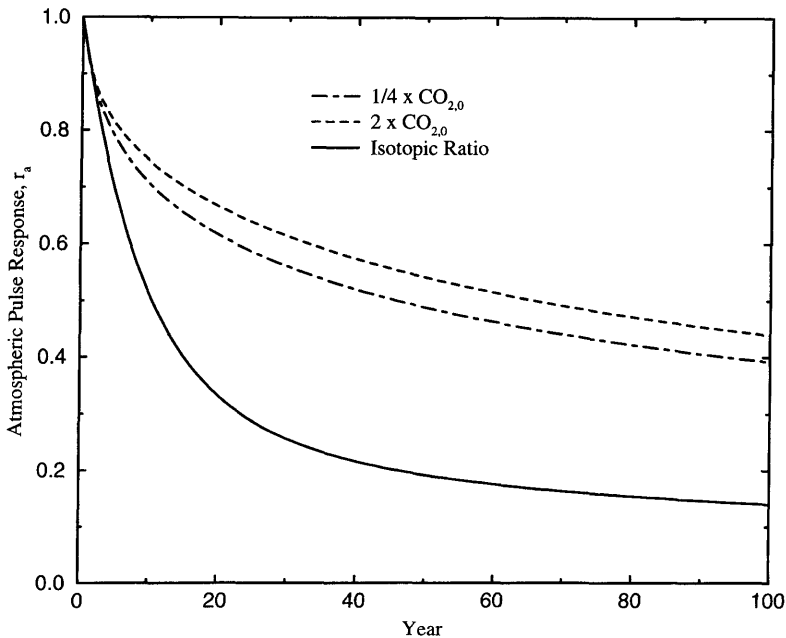
Fig. 1. Atmospheric pulse response functions for an isotopic ratio ( 13 C/ 12 C or 14 C/ 12 C) and for CO 2 as obtained by using the ocean-atmosphere compartments of the HILDA model with no biosphere. The response of the atmospheric CO 2 concentration to a pulse input depends on the pulse size and the CO 2 background concentration. The dashed line is for a doubling of preindustrial CO 2 concentration (280 ppm) at t = 0 ; the dashed-dotted line is for an increase of pre-industrial CO 2 concentration by one quarter (70 ppm) at t = 0 ; the solid line is for the decrease of an isotopic perturbation.
